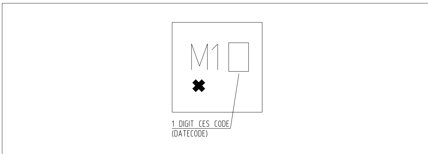
Figure 3: Marking Specification (top view)
